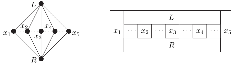
Fig. 3. A 5-rung ladder (dotted lines indicate paths) and a possible layout. In any layout, all the x_i must be stacked, and the rectangles x_2 , x_3 , and x_4 must be aligned as shown between L and R . The only other variations also align rectangle(s) x_1 and/or x_5 , but the width remains at least 5.
