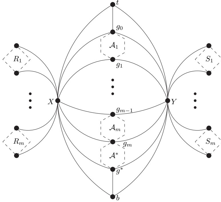
Fig. 10. The graph G(\mathcal{I}) for some instance \mathcal{I} of numerical matching with target sums. The accordions are denoted by dashed hexagons and the ladders by dashed diamonds.
