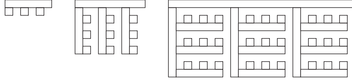
Fig. 8. Layouts L_3^3 (left), L_9^3 (middle), and L_{27}^3 (right).
