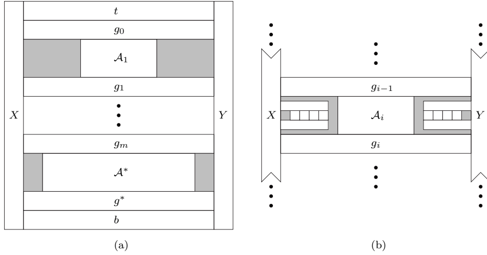
Fig. 11. (a) An incompressible sub-layout for G(\mathcal{T}) . (b) Filling the gaps in layer i by some R_i and S_i .
