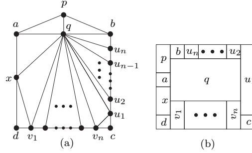
Fig. 12. (a) A graph on 2n + 7 vertices. (b) A rectangular dual of area 6(n + 2) .
