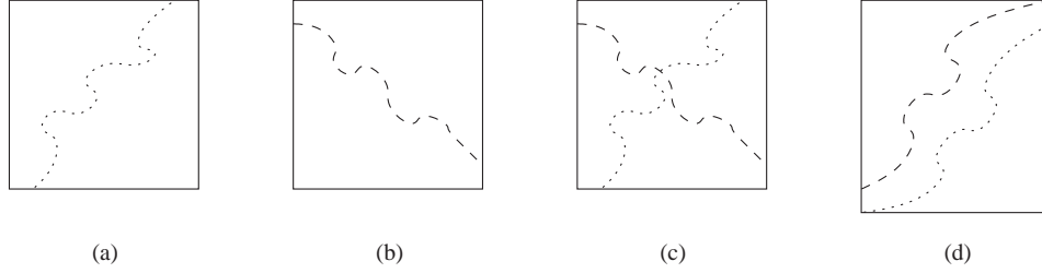
Fig. 6. Bounding boxes and extremal paths for various layouts. (a) Layout L_1 for G_1 ; (b) Layout L_2 for G_2 ; each of size d -by- d . (c) Impossible d -by- d layout for G containing G_1 and G_2 as subgraphs; any corresponding extremal paths would have to cross. (d) d -by- (d+1) layout for G . The extremal path for L_1 is dotted, and that for L_2 is dashed. By extending G in one dimension, the extremal paths need not cross.
