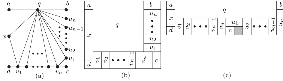
Fig. 13. (a) The graph on 2n + 6 vertices derived by deleting vertex p from Figure 12(a). (b) A rectangular dual of area (n + 3)(n + 2) . (c) A strong rectangular layout of area 4(n + 2) .
