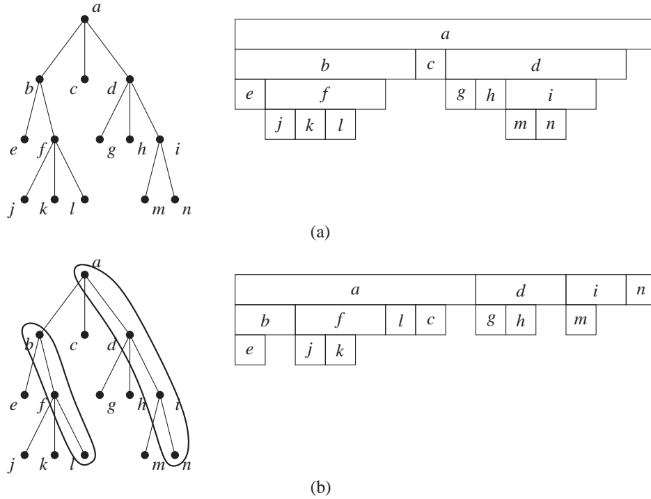
Fig. 5. (a) A tree and the result of applying Algorithm A. The width of each rectangle is the number of descendants of the corresponding vertex; e.g., the width of f is 4, and the width of d is 6. (b) A partition of the tree into paths—uncircled nodes form singleton paths—and the application of Algorithm B to the partition.
