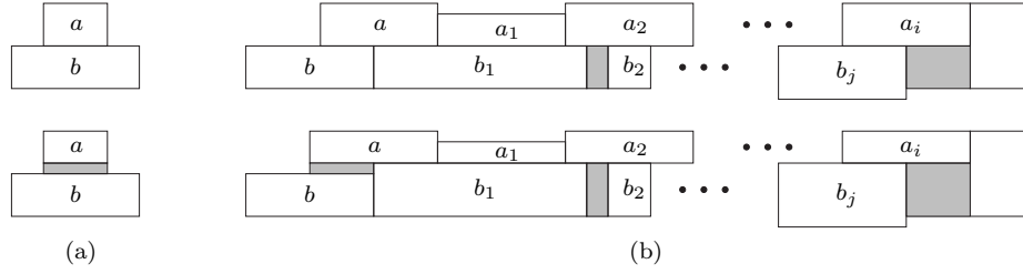
Fig. 2. Weak layouts (top) and corresponding strong layouts (bottom) after fixing the \{a, b\} violation. (a) The violating boundary of a is nested in that of b . (b) No nesting occurs; shear the projection of the violating boundary until hitting a blocking rectangle. In both cases, there can be other rectangles not shown, but if the new separation \epsilon is less than the smallest prior boundary overlap, no other adjacencies are broken.
