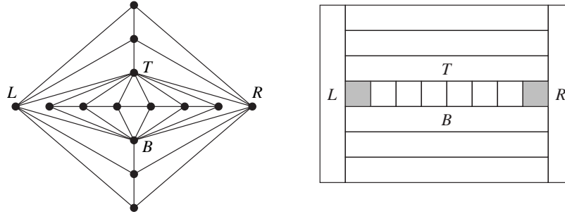
Fig. 4. A (6,6)-ladder and a possible layout.
