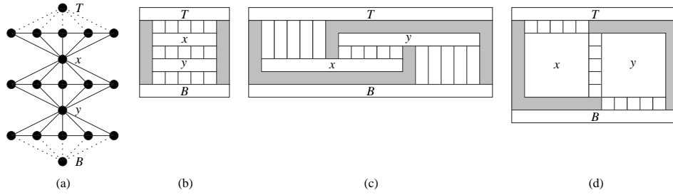
Fig. 9. (a) A 5-accordion enclosed by T and B . The accordion edges are solid; the enclosing edges are dotted. (b)–(d) Layouts with (b) y below x ; (c) x below y ; and (d) neither x nor y below the other.
