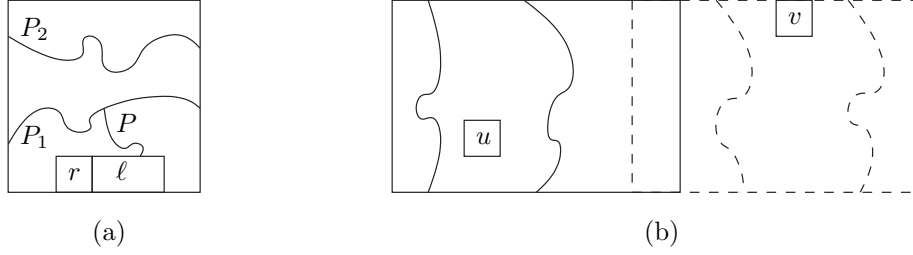
Fig. 7. (a) A bounding box of width d containing a layout L that includes two sub-layouts L_1 and L_2 , each of minimum dimension d . If r is adjacent to the bottom of L , let \ell be a rectangle in L_1 adjacent to r . There is some path P in L_1 connecting \ell to a horizontal extremal path P_1 of L_1 and L . No horizontal extremal path of L_2 can intersect the closed curves formed by P , P_1 , and the bounding box of L . Thus P_2 is above P_1 , but then r cannot be connected to P_2 without crossing P_1 . (b) Bounding boxes for layouts of two T_{i-1} 's, rooted at u (solid) and v (dashed). If both layouts are of height \lfloor \frac{i-2}{2} \rfloor , then extremal paths (dashed for the T_{i-1} rooted at v ) separate u from v , and r cannot be placed within this height.
